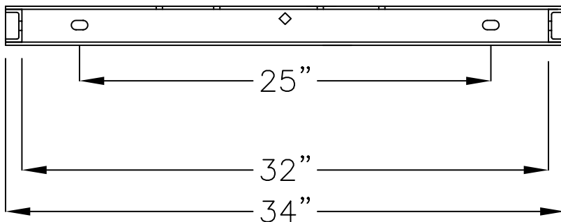
RAIL BRACKET FRONT
